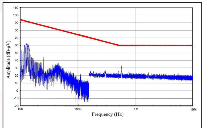
Figure 24: High frequency conducted emissions of MQHL-28-05S, 5V out module at 50W output with MQHE-28-P filter, as measured with Method CE102. Limit line shown is the 'Basic Curve' for all applications with a 28V source.
