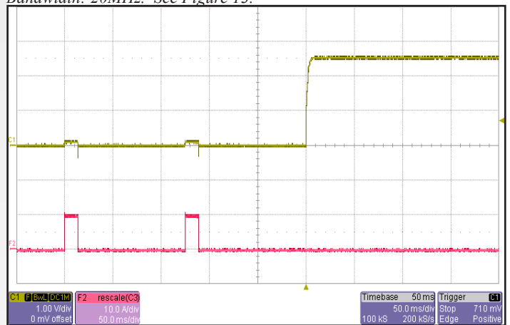
Figure 16: Rise of output voltage after the removal of a short circuit across the output terminals. Ch 1: V_{out} (1V/div). F 2: I_{out} (10A/div).
