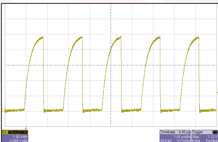
Figure 17: SYNC OUT vs. time, driving SYNC IN of a second SynQor MQBL converter. Ch1: SYNC OUT: (1V/div).
