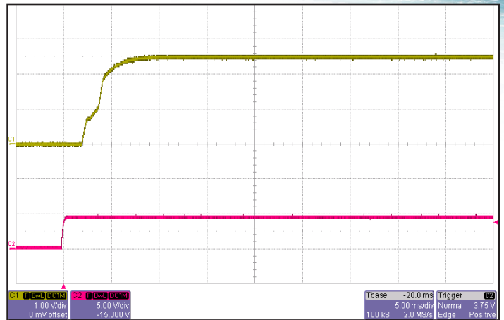
Figure 8: Turn-on transient at full resistive load and 2mF output capacitance initiated by ENA1. Input voltage pre-applied. Ch 1: Vout (1V/div). Ch 2: ENA1 (5V/div).
